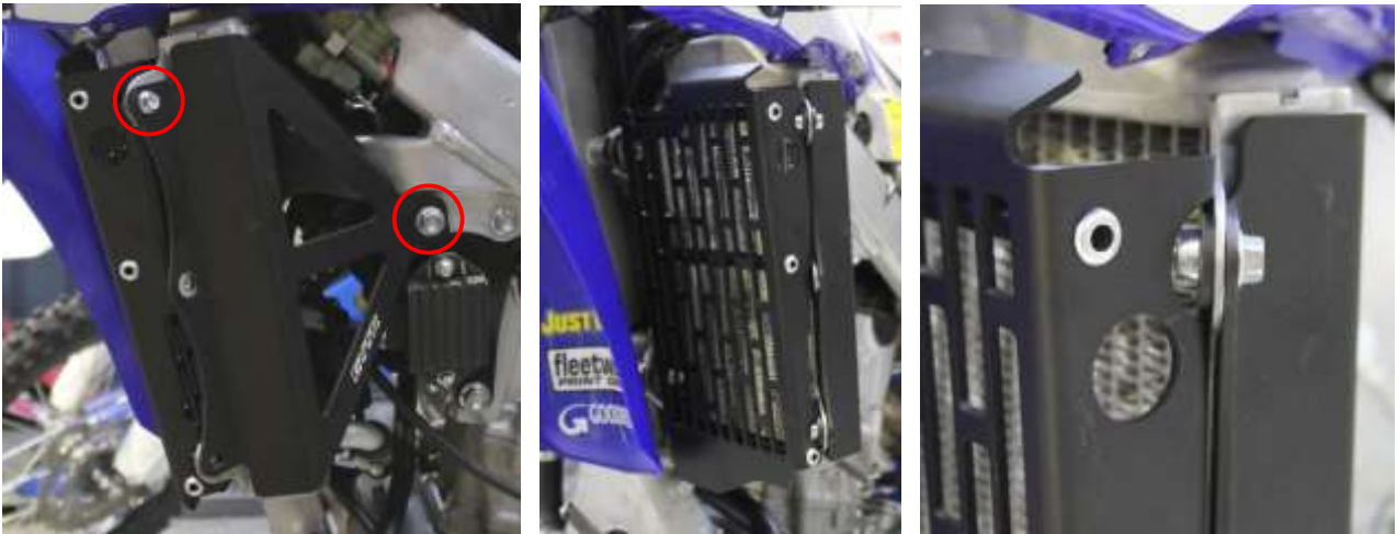
Figure 3: Fitted guards and braces, ready for the lower radiator shrouds to go back on
